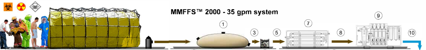
Typical decon station with decon runoff transferred to holding bladder
